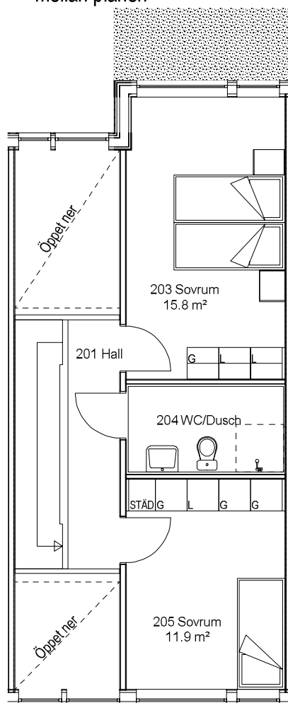
PLAN 2
